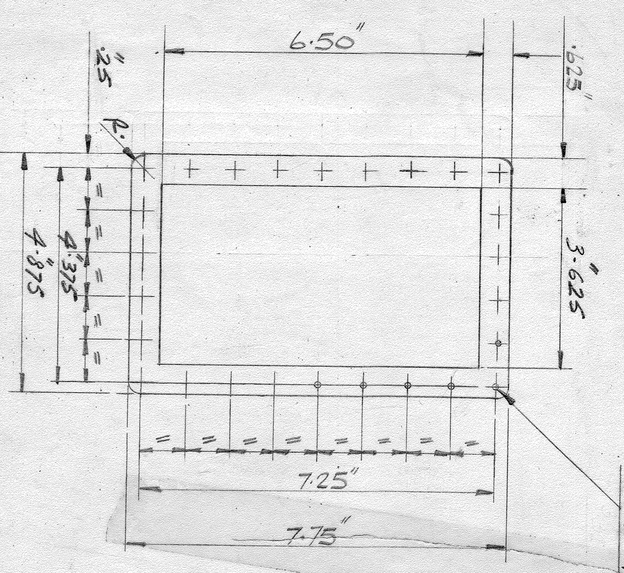
DETAIL - ITEM 6
